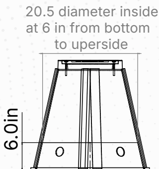
SECTION VIEW
