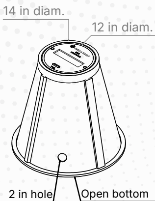
ISOMETRIC VIEW
