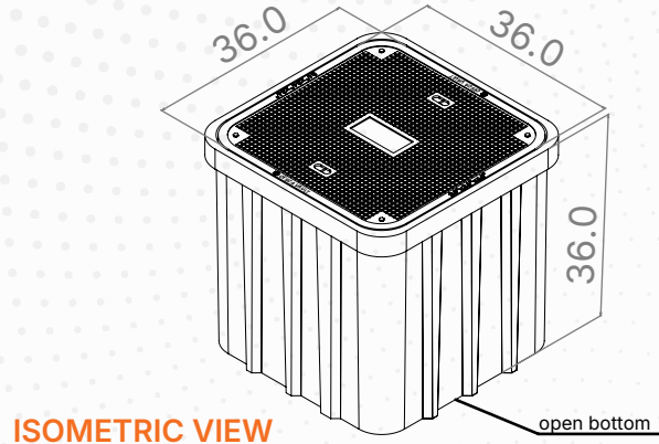
ISOMETRIC VIEW
